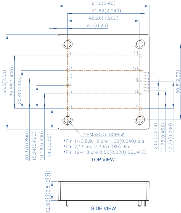
Without flange
