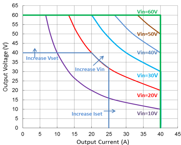
Figure 1. Typical V-I Characteristic in Boost Mode
