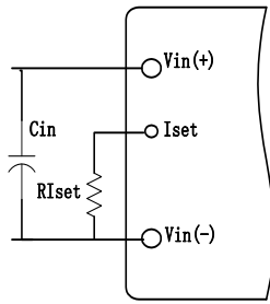
Figure 6. Circuit to Program Output Current Set Point
