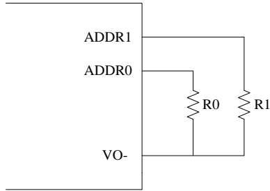
Figure 8. Address-configure Resistors
