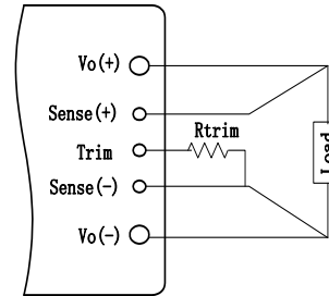
Figure 5. Circuit to Program Output Voltage Set Point
