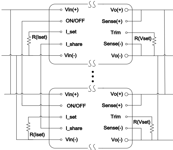
Figure 7. Circuit Configuration for Active Current Share
